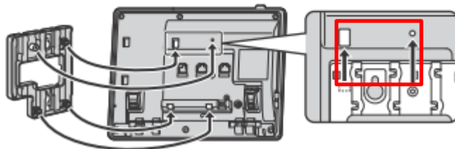
KX-HDV230N
